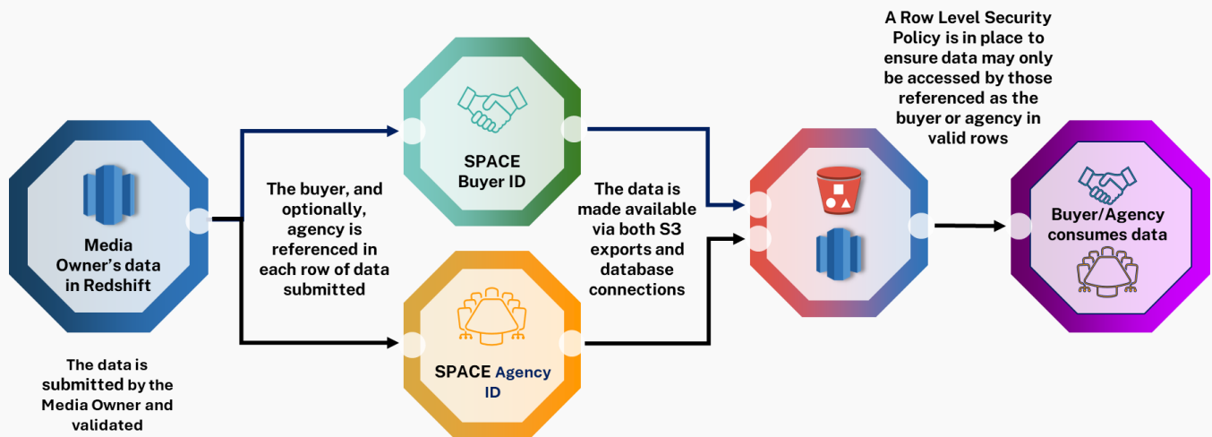
Fig. 2: The Playout Security Model
